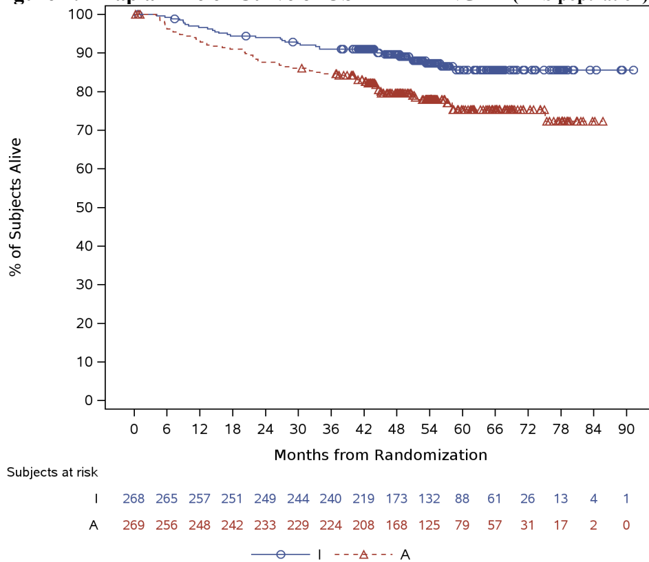
Figure 2: Kaplan-Meier Curve of OS § in TRIANGLE (FAS population)*
