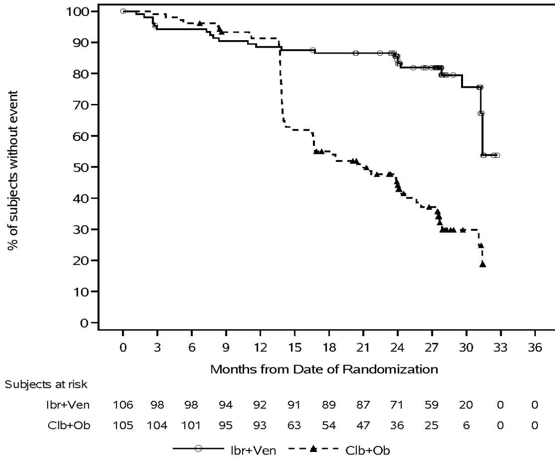
Figure 9: Kaplan-Meier Curve of Progression-Free Survival (ITT Population) in Patients with CLL in Study CLL3011
