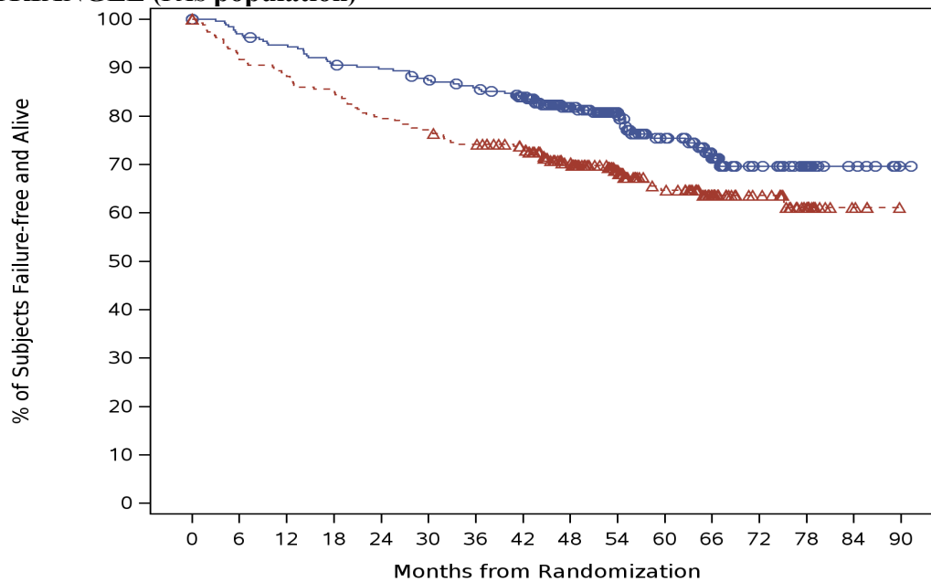
Figure 1: Kaplan-Meier Curve of European MCL Network Assessed Failure-free Survival in TRIANGLE (FAS population) *
