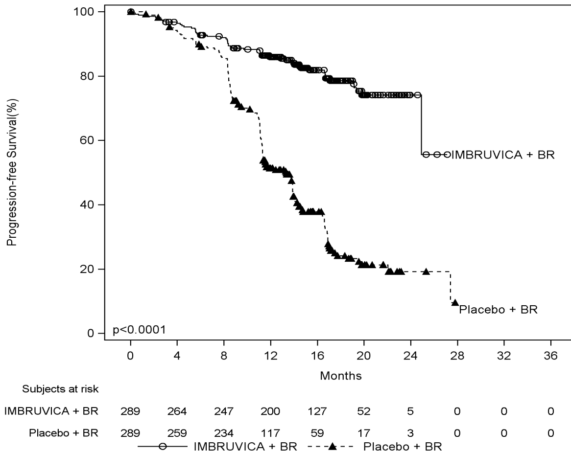
Figure 6: Kaplan-Meier Curve of Progression-Free Survival (ITT Population) in Patients with CLL/SLL in HELIOS
